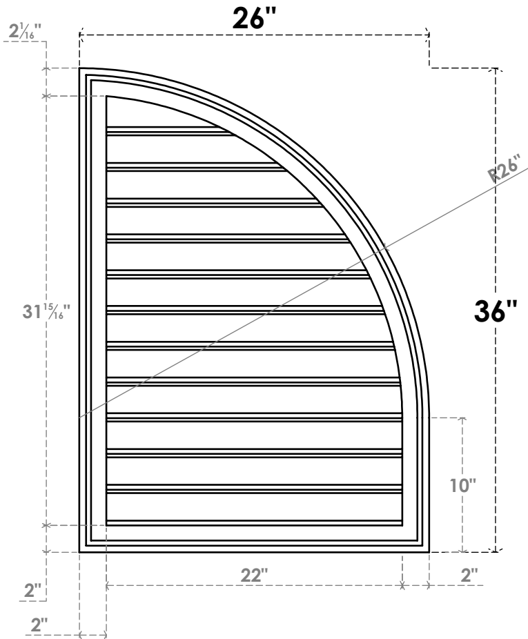
FRONT
